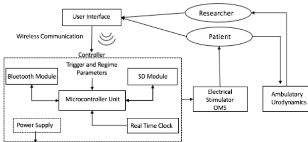
Figure 2. Block diagram of system outlining components and interactions relative to both patient and researcher
