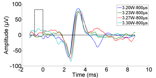
Figure 3. Measurements of muscle action potentials triggered by photonic stimulation in a mouse. The black dotted line represents the photonic pulse duration of 800 μs. The signals are smoothed by a moving average filter (Matlab function 'smooth').
