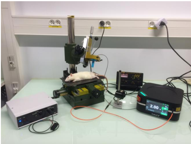
Figure 2. Photonic stimulation set-up - From left to right: the NDP_V1 with two stimulating electrodes, the milling support with a rat on the heating plate and the cannula pointed towards its leg, the power meter and the neoV laser.
