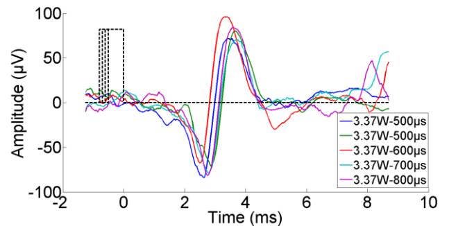
Figure 4. Measurements of muscle action potentials triggered by photonic stimulation in a mouse. The black dotted lines represent the photonic pulse duration, which varies from 500 μs to 800 μs. The signals are smoothed by a moving average filter (Matlab function 'smooth').
