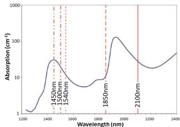
Figure 1. Water absorption between 1200 nm and 2400 nm. The marked wavelengths are those often used in the literature to stimulate neuronal membranes (sensory or motor neurons or axons). Pertinent authors are listed here: [5], [4], [9] between 1455 nm and 1550 nm, [10], [11], [12], [13], [14], [15] between 1844 nm and 1875 nm (laser diodes from Aculight) and [16], [17], [18] at 2120 nm (Ho:YAG laser). Figure adapted from McCaughey et al. [4].
